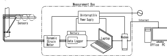
Fig.4 System of Measurement
