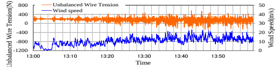
Fig.8 Unbalanced Wire Tension (Time Series Data)
