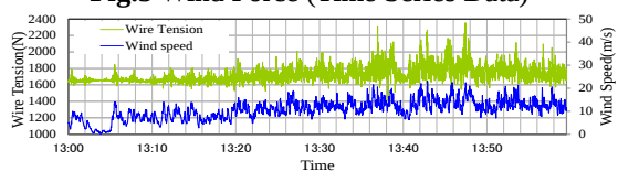
Fig.6 Wire Tension_Left Side (Time Series Data)
