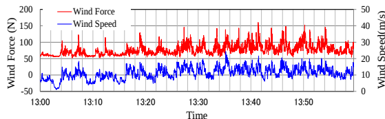
Fig.5 Wind Force (Time Series Data)
