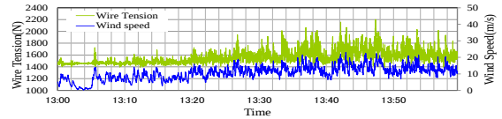
Fig.7 Wire Tension_Right Side (Time Series Data)
