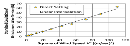
Fig.9 \bar{V}^2 vs \sigma_u
