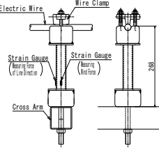
Fig.3 Bending Strain Sensor
