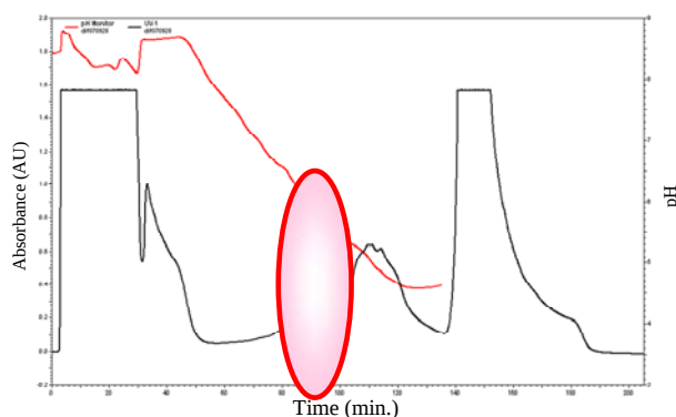
Fig.1. 1st Dimension-HPLC using PF2D
