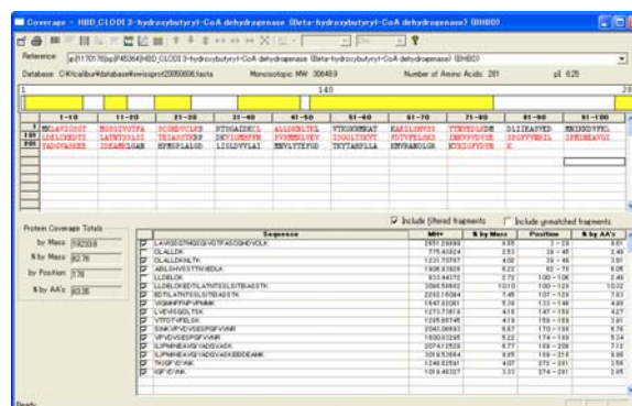
Fig.2. Result of Mass Spectrometry
