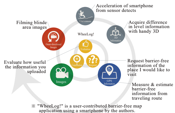
Fig.1 Overview of "WheelLog!"
