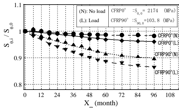
Fig.6 Comparison with flexural strength ratios of analysis to experimental ones under steady load and no load of outdoor exposure for CFRP0° and 90°
