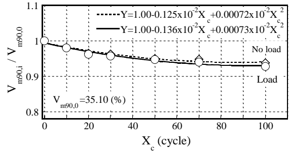
Fig.2 Results of matrix volume fraction ratio under steady load and no load of accelerated exposure for CFRP90°
