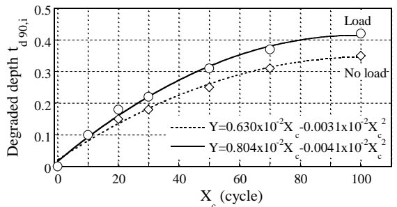
Fig.3 Results of degraded depth under steady load and no load of accelerated exposure for CFRP90°
