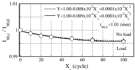
Fig.4 Results of thickness ratio under steady load and no load of accelerated exposure for CFRP90°
