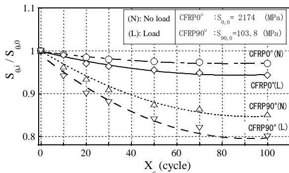
Fig.5 Comparison with flexural strength ratios of analysis to experimental ones under steady load and no load of accelerated exposure for CFRP0° and 90°
