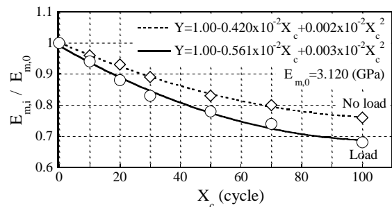
Fig.1 Results of flexural modulus ratio under steady load and no load of accelerated exposure for EP
